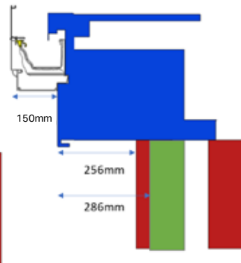
Flat Cornice
