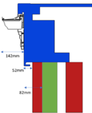
Classic Fascia
