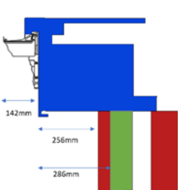
Classic Fascia
