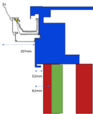
Curved Cornice
