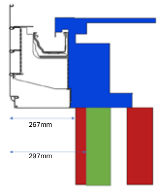
Four Tier Cornice
