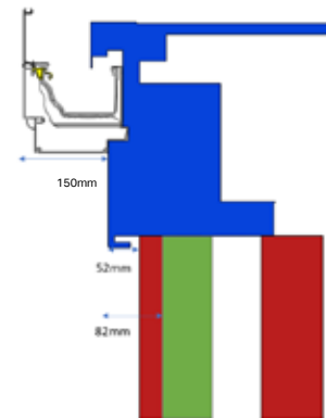
Flat Cornice
