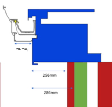
Curved Cornice
